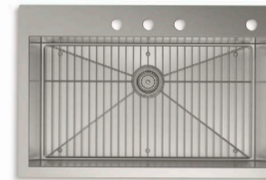
Vault™ TOP-MOUNT/UNDERMOUNT Includes sink rack. 33" x 22" x 9" | K-3821 (shown) 25" x 22" x 9" | K-3822 25" x 22" x 6" | K-3894
